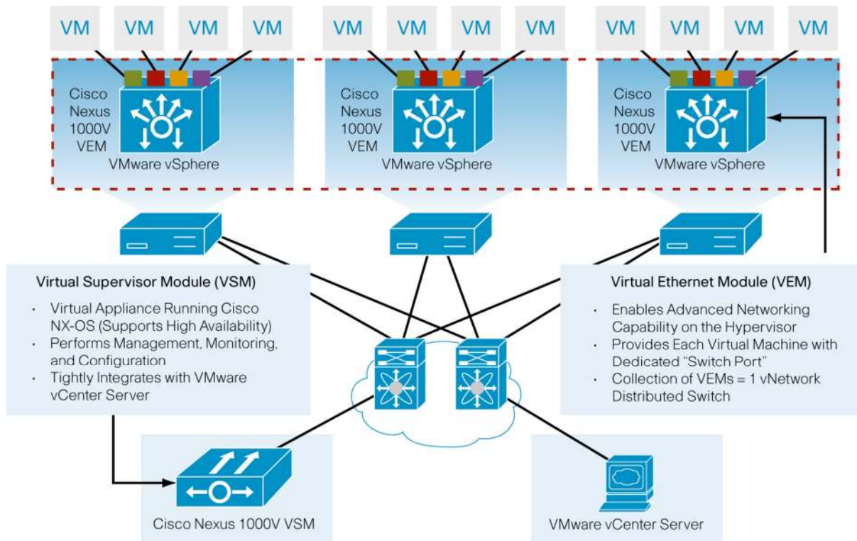
Figure 2. Cisco Nexus 1000V Series Architecture
