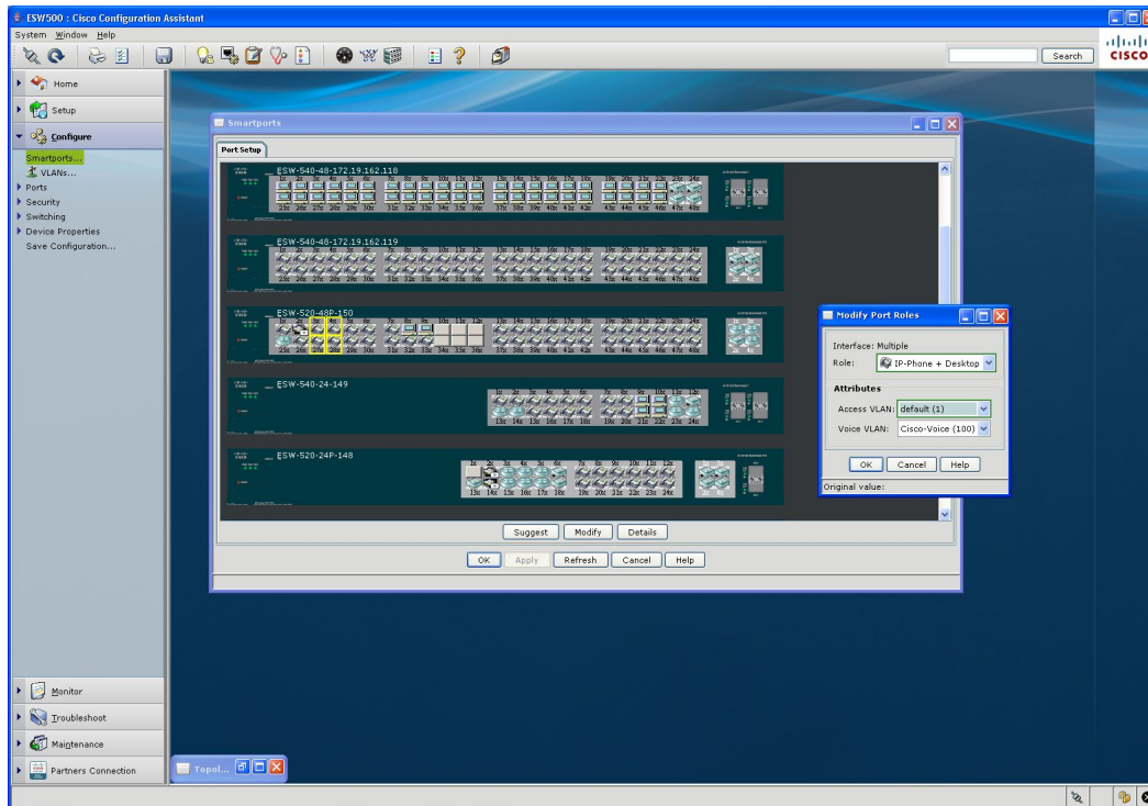
Figura 4. Cisco Configuration Assistant: vista del panel frontal
